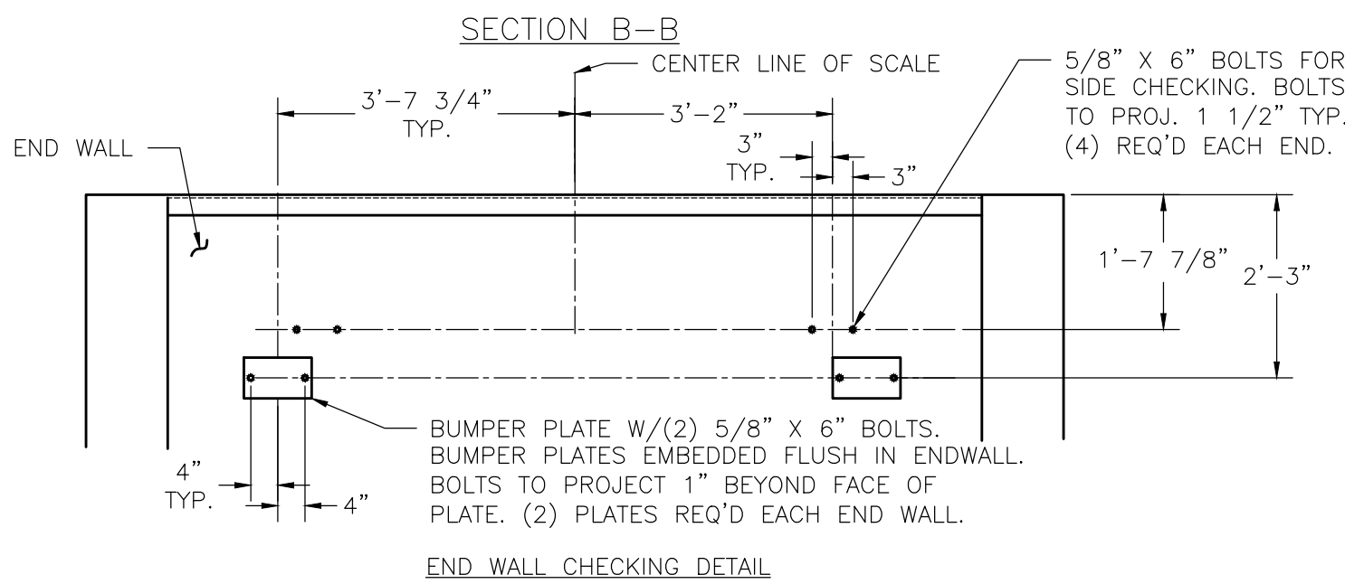
END WALL CHECKING DETAIL
