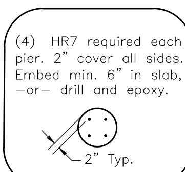
SAFETY PIER REINFORCING Top View
