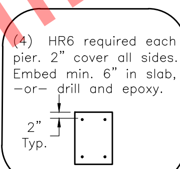
PIER REINFORCING Top View
